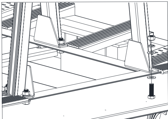
M14 bolt x 40 mm attach upwards
